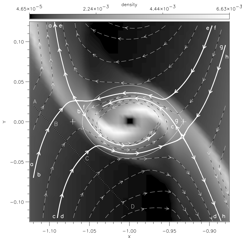
FIG. 4.—A high-resolution density image (in Cartesian coordinates) of the Roche lobe region about a 1 M_J planet. The planet is at location x = -1 , y = 0 , and the star is located at the origin. The left (right) plus sign marks the L_2 ( L_1 ) point. Sample streamlines are dashed flow lines. Critical streamlines that separate distinct flow regions are solid flow lines (see § 4.3). The dotted line segment AD is used for Fig. 6.
