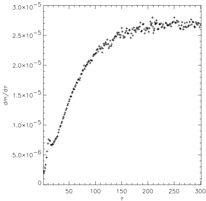
FIG. 3.—Mass accretion rate onto a 1 M_J planet versus time. The accretion rate is expressed in units of the disk mass M_d per planetary orbit, and the time is in units of planetary periods. Each point represents the mass accretion rate averaged over one planetary orbit.
