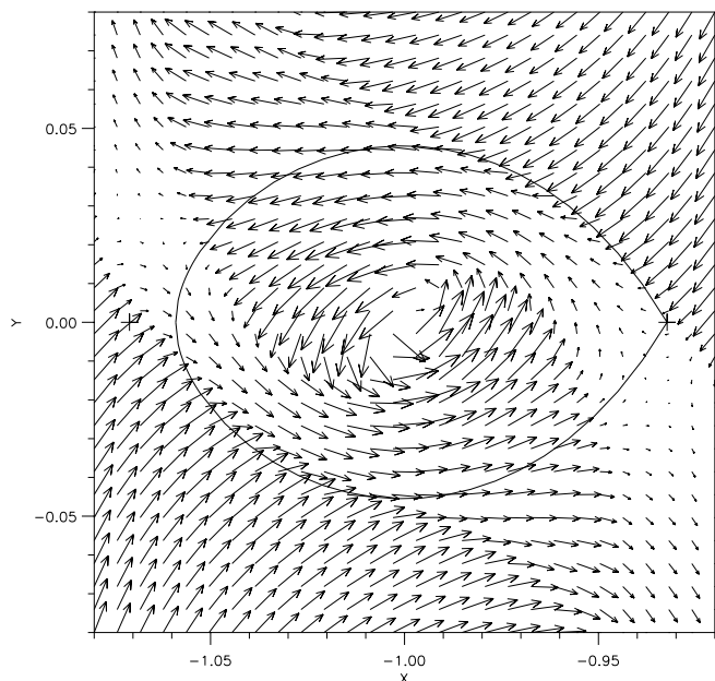
FIG. 5.—A high-resolution velocity map in the corotating frame of the planet (in Cartesian coordinates) of the Roche lobe region about a 1 M_J planet. The planet is at location x = -1 , y = 0 , and the star is located at the origin. The left (right) plus sign marks the L_2 ( L_1 ) Lagrangian point (see § 4.3).
