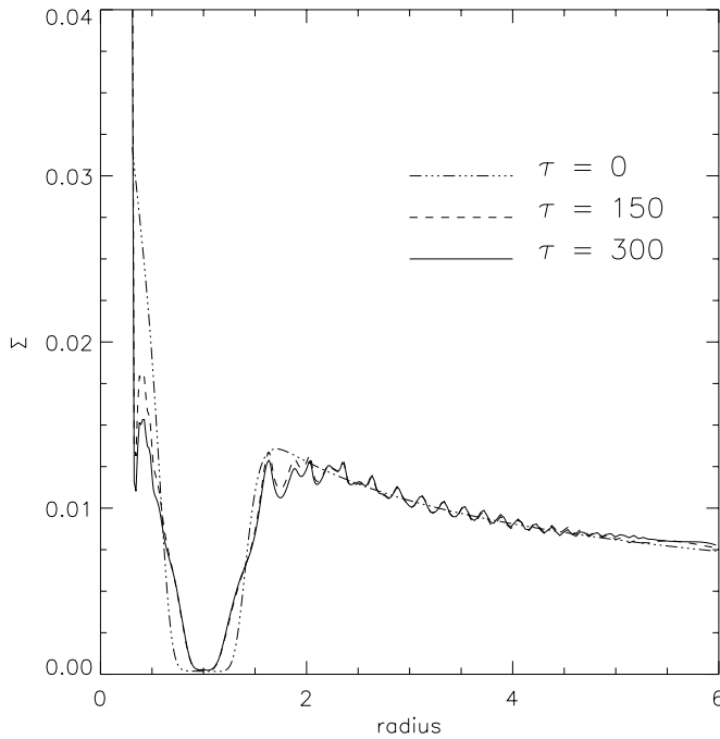
FIG. 1.—Azimuthally averaged surface-density profiles of a disk containing a planet at various times. Density is normalized by M_d/a^2 , where M_d is the simulated disk mass and a is the planetary orbital radius. The horizontal axis is normalized by a . A 1 M_J planet resides at r = 1 , and a 1 M_\odot star is located at r = 0 . The disk properties are described in § 4.1. The dash-dotted line is the initial density profile, the dashed line is the profile at 150 planetary orbits, and the solid line is the profile at 300 planetary orbits.
